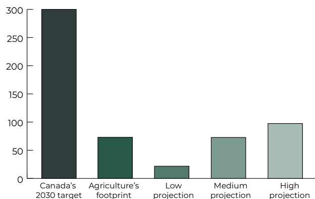
Figure 11: Potential Impact on Canada’s 2030 GHG Reduction Targets (Megatonnes CO 2e /yr)
