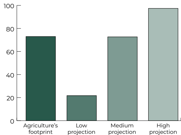
Figure 11: Potential Impact on Canada’s 2030 GHG Reduction Targets (Megatonnes CO 2e /yr)
